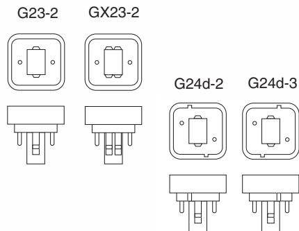
(3) 2-Pin Base
