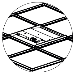
T-Grid Mount
