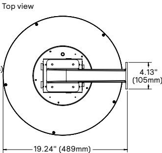
Wall mount
