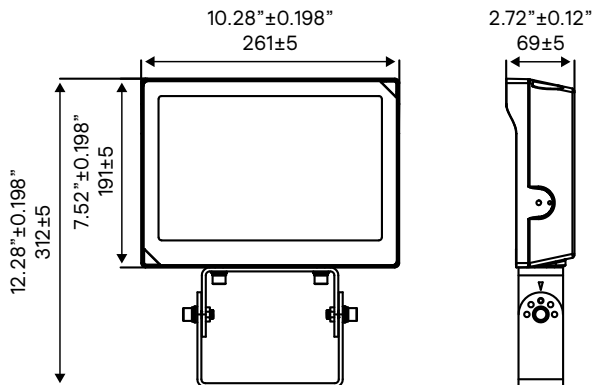
100W Trunnion Slim Flood 60–80–100W/3CCT/UN3/TN/PCB
