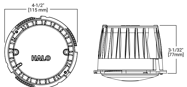
120-277V - 0-10V dimming
