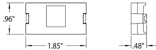
41291-1Mx, 41291-2Qx (1 unit high)
