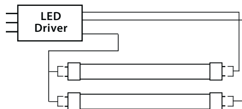
2 Lamp T8 System
