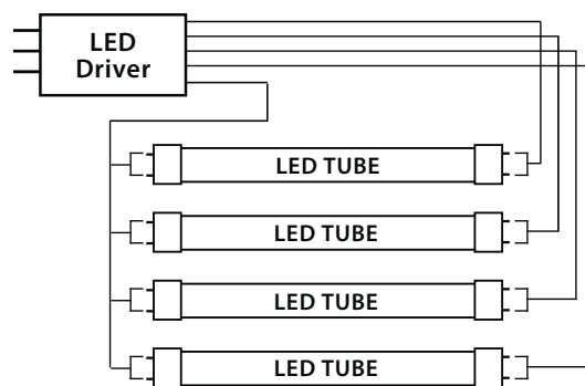
4 Lamp T8 System
