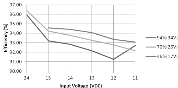
Efficiency - Input vs. Load
