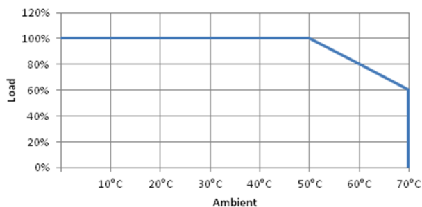
Derating Temp. vs. Load
