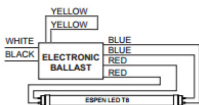
1-LAMP Programmed Start Electronic Ballast
