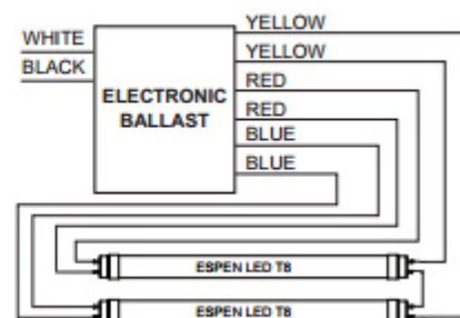
2-LAMP Programmed Start Electronic Ballast
