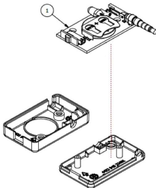
Figure 2 Assemble the parts
