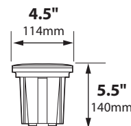
(2) 1/2" NPS threaded ports available on bottom
