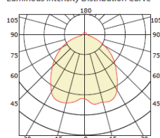
Conical Bottom Lens Luminous Intensity Distribution Curve
