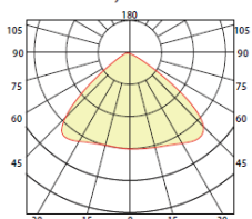
120 Degree lens Luminous Intensity Distribution Curve
