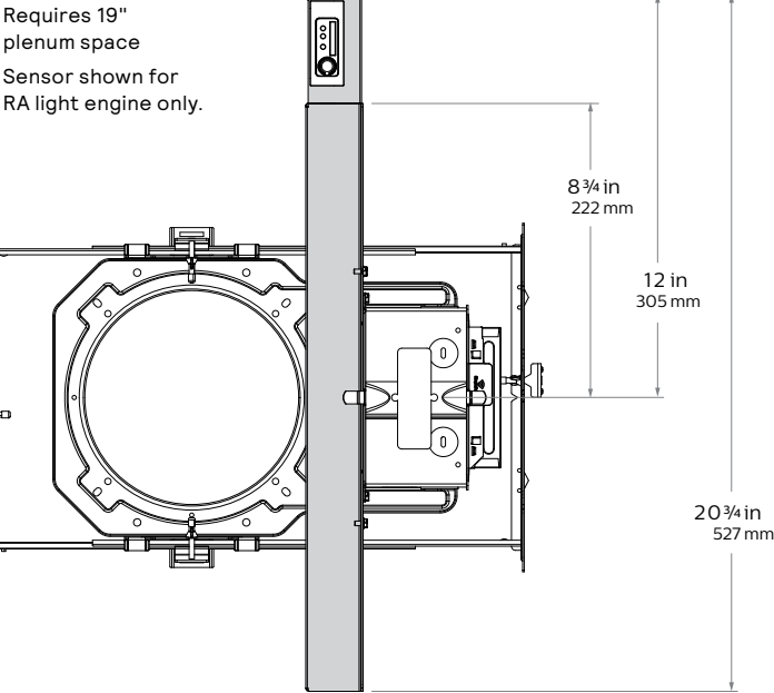
Surface/Pendant Remote Driver (driver assembly recessed into ceiling)
