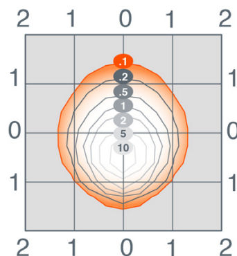
150W BULLTFL1A/15UNV740MFBZ 10' setback with 30° tilt
