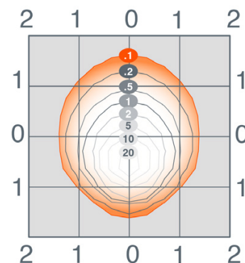
20W BULLTFL1A/20UNV740MFBZ 10' setback with 30° tilt
