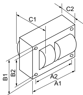
MH BAL 400W M59 5-TAP KIT
