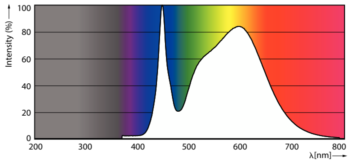
Spectral Power Distribution Colour - 115CC/LED/840/LS EX39 G2 BB 3/1
