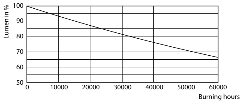
Lumen Maintenance Diagram - 115CC/LED/840/LS EX39 G2 BB 3/1
