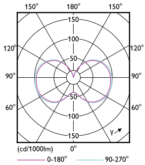
Light Distribution Diagram - 115CC/LED/840/LS EX39 G2 BB 3/1
