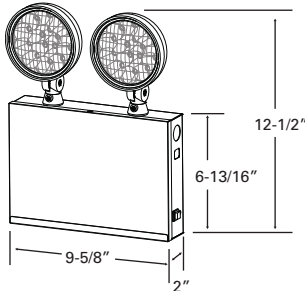
10-REL36-LED42
