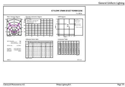
General uniform lighting - 0.5C7/LEDnight light/E12/MilkyND120V 2PF
