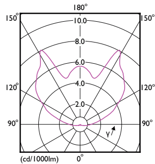
Light Distribution Diagram - 0.5C7/LEDnight light/E12/MilkyND120V 2PF
